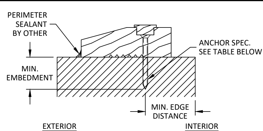
U18 INSTALLATION DETAIL INSWING DOOR SILL
