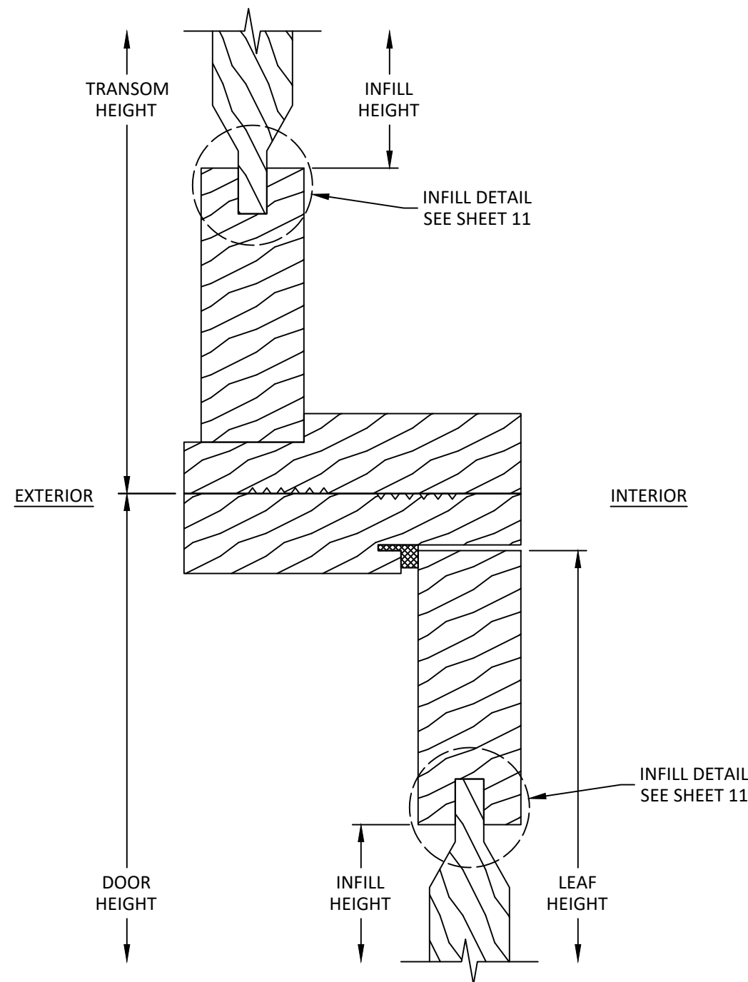
VERTICAL SECTION TRANSOM TO DOOR INSWING SHOWN, OUTSWING SIMILAR TRANSOM TO SIDELITE SIMILAR
