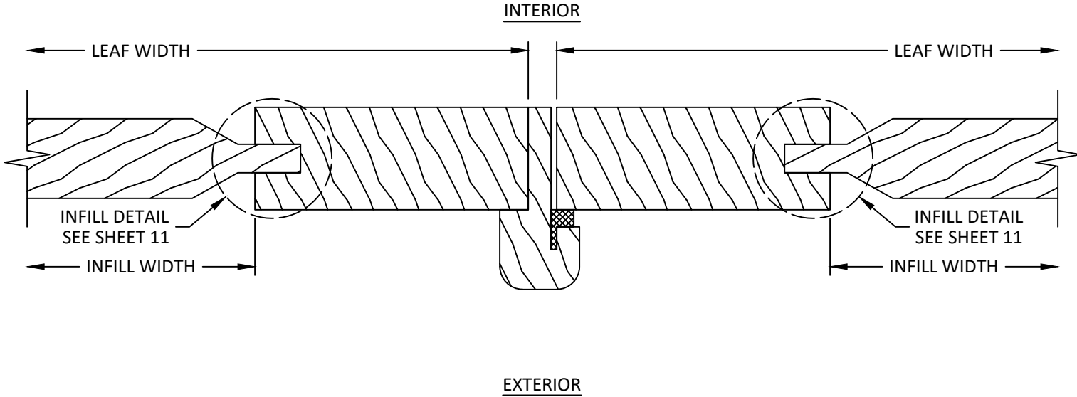
L 15 HORIZONTAL SECTION INSWING DOOR ASTRAGAL
