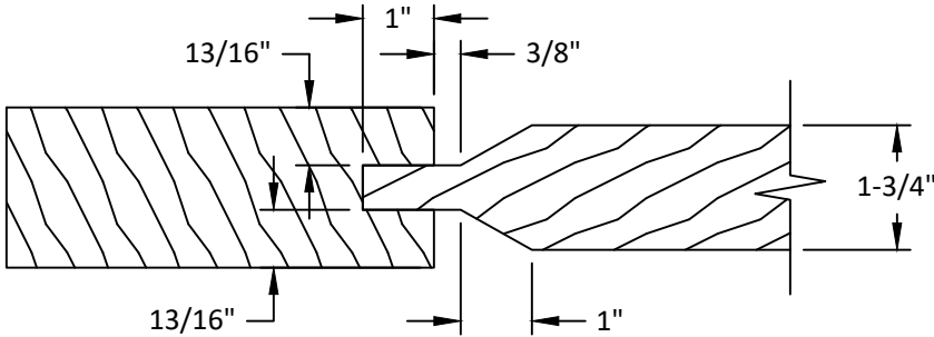
INFILL DETAIL
