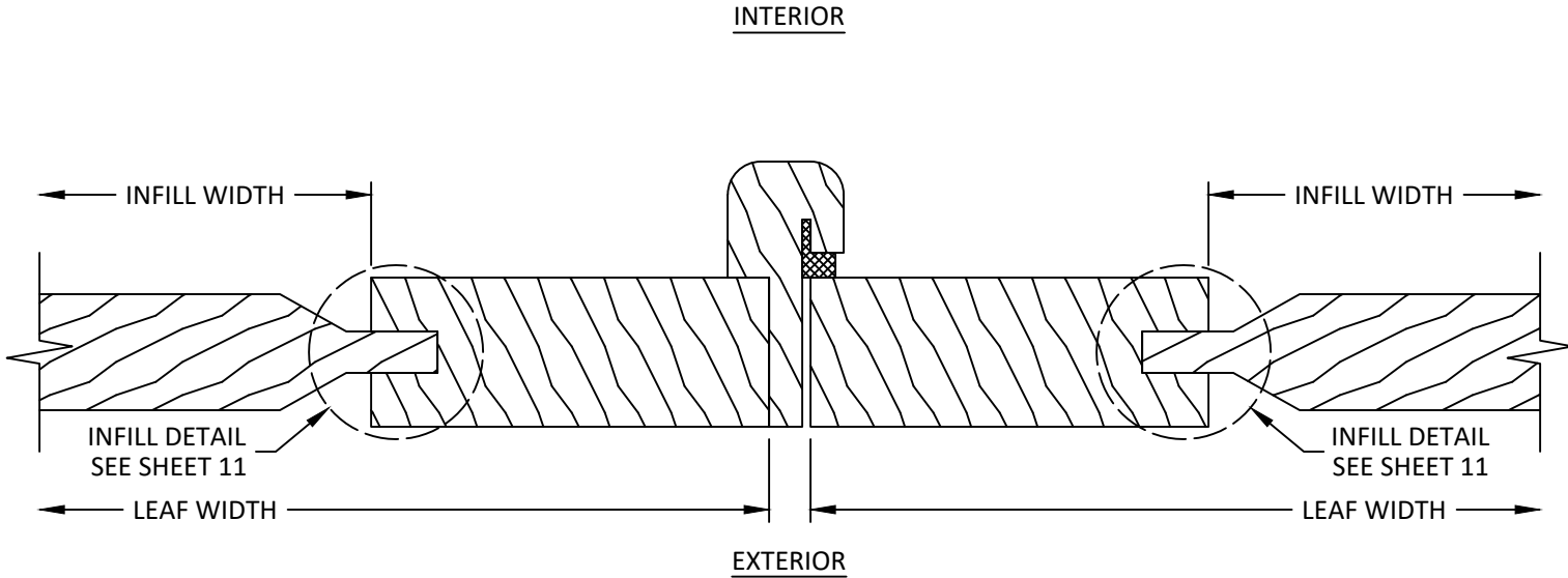
N 15 HORIZONTAL SECTION OUTSWING DOOR ASTRAGAL
