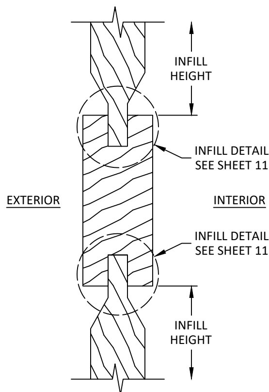
VERTICAL SECTION
