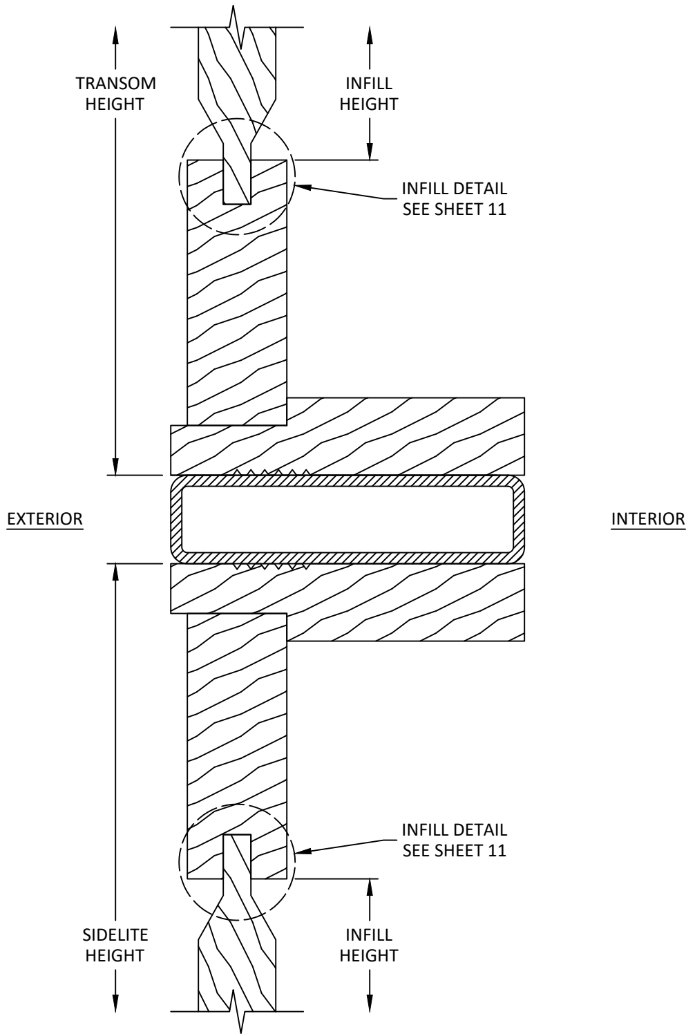
I 14 VERTICAL SECTION TRANSOM TO SIDELITE W/ ALUM. MULLION INSWING SHOWN, OUTSWING SIMILAR
