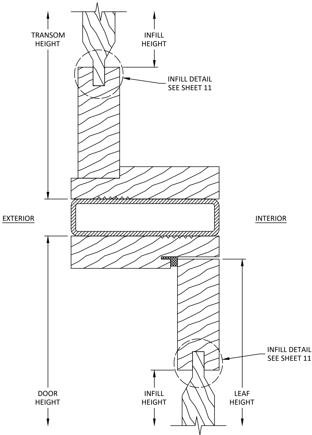
J 14 VERTICAL SECTION TRANSOM TO DOOR W/ ALUM. MULLION INSWING SHOWN, OUTSWING SIMILAR
