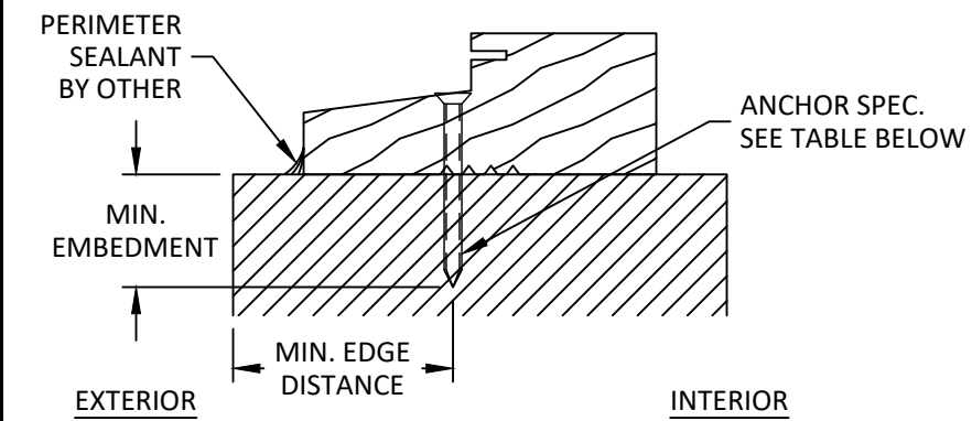
V18 INSTALLATION DETAIL OUTSWING DOOR SILL
