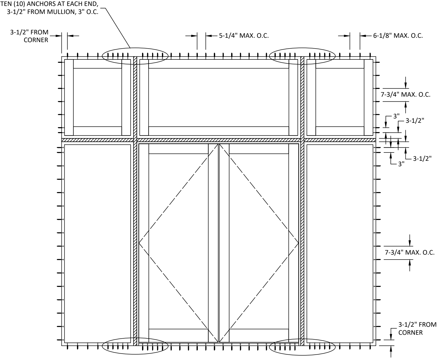
ANCHOR LAYOUT DOUBLE DOOR W/ SIDELITE & TRANSMOM SINGLE DOOR SIMILAR
